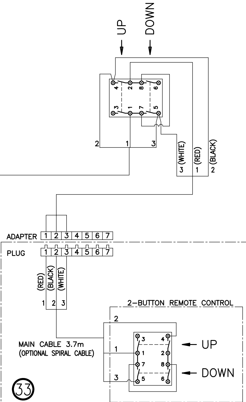
ELECTRICAL WIRING DIAGRAM ATKM16B
