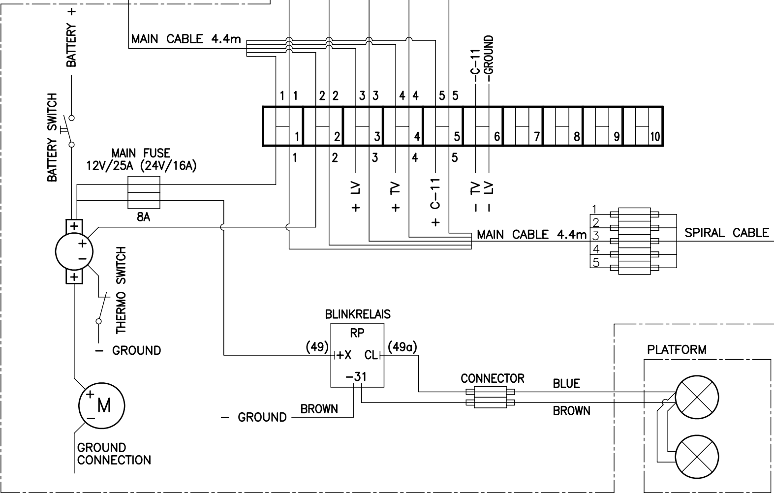
31 ELECTRICAL WIRING DIAGRAM LSMB2BWC
