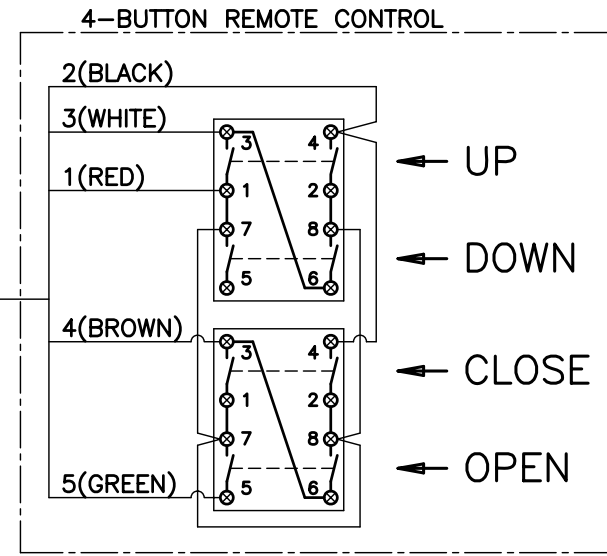
31 ELECTRICAL WIRING DIAGRAM LSMB2BWC
