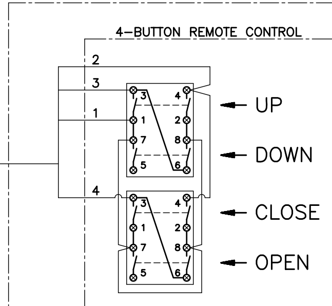
ELECTRICAL WIRING DIAGRAM LSM12BC; LSM12BDC
